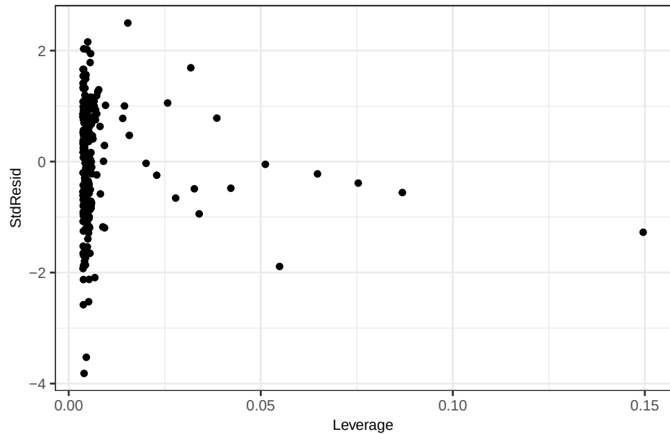
Ca WLS – Leverage Plot
